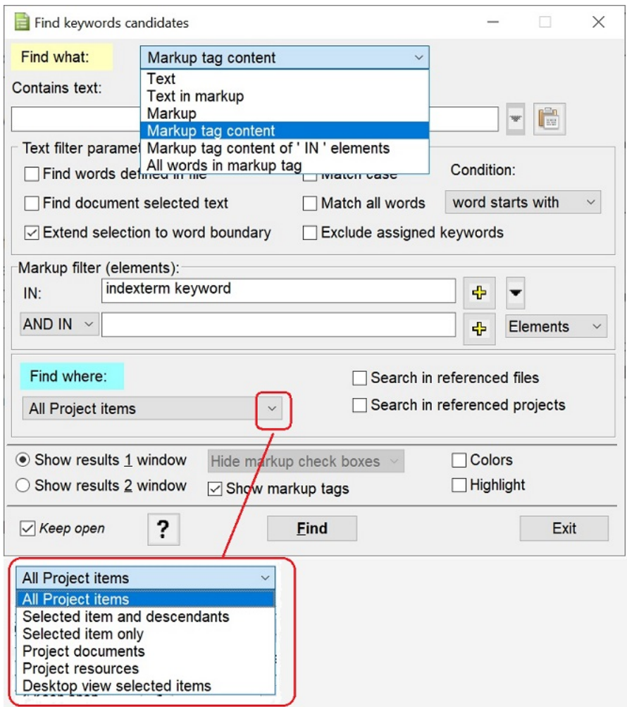
Figure 17: Find keywords candidates: UI
