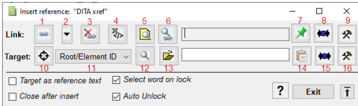
Figure 10: Insert reference: default UI
