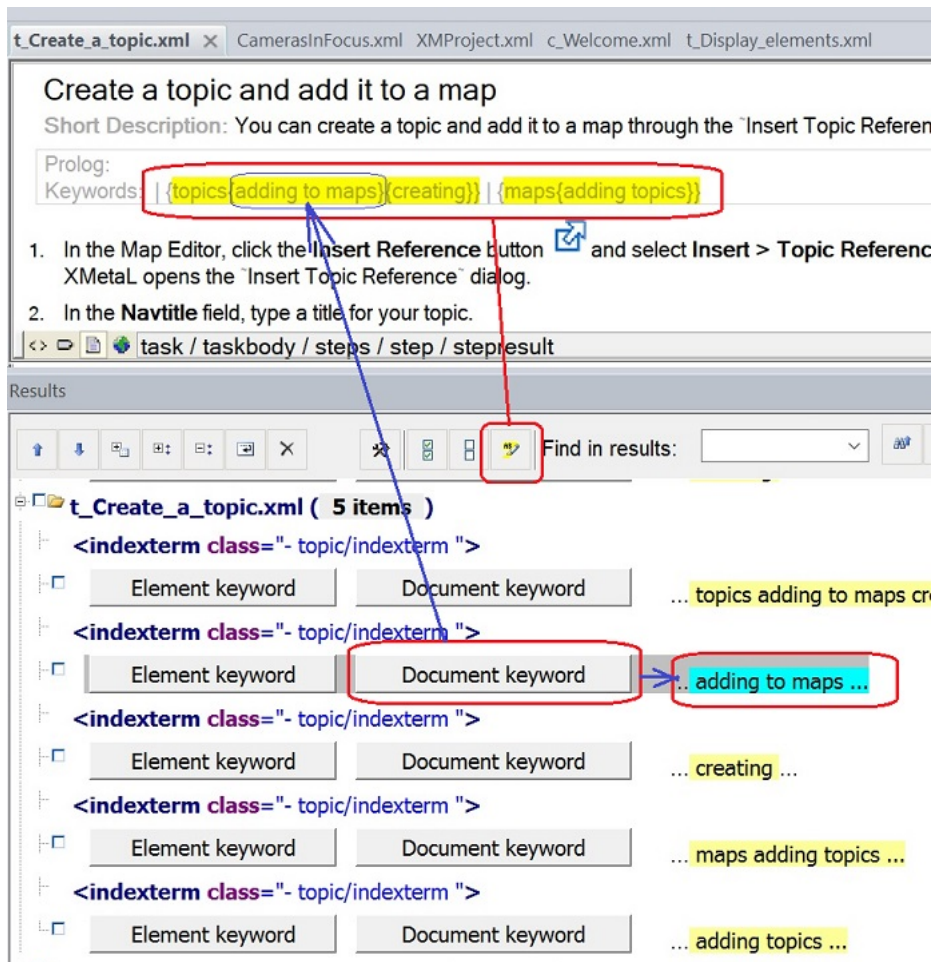
Figure 18: Find keywords candidates: Set keyword from results tab
