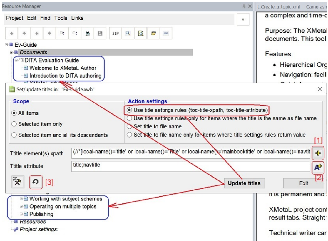
Figure 1: Set/Update titles: User Interface
