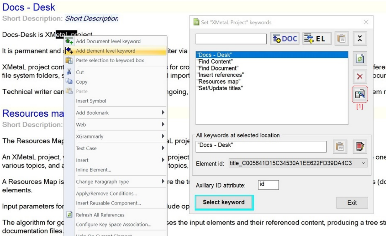
Figure 16: Set keywords full user interface and context menu example
