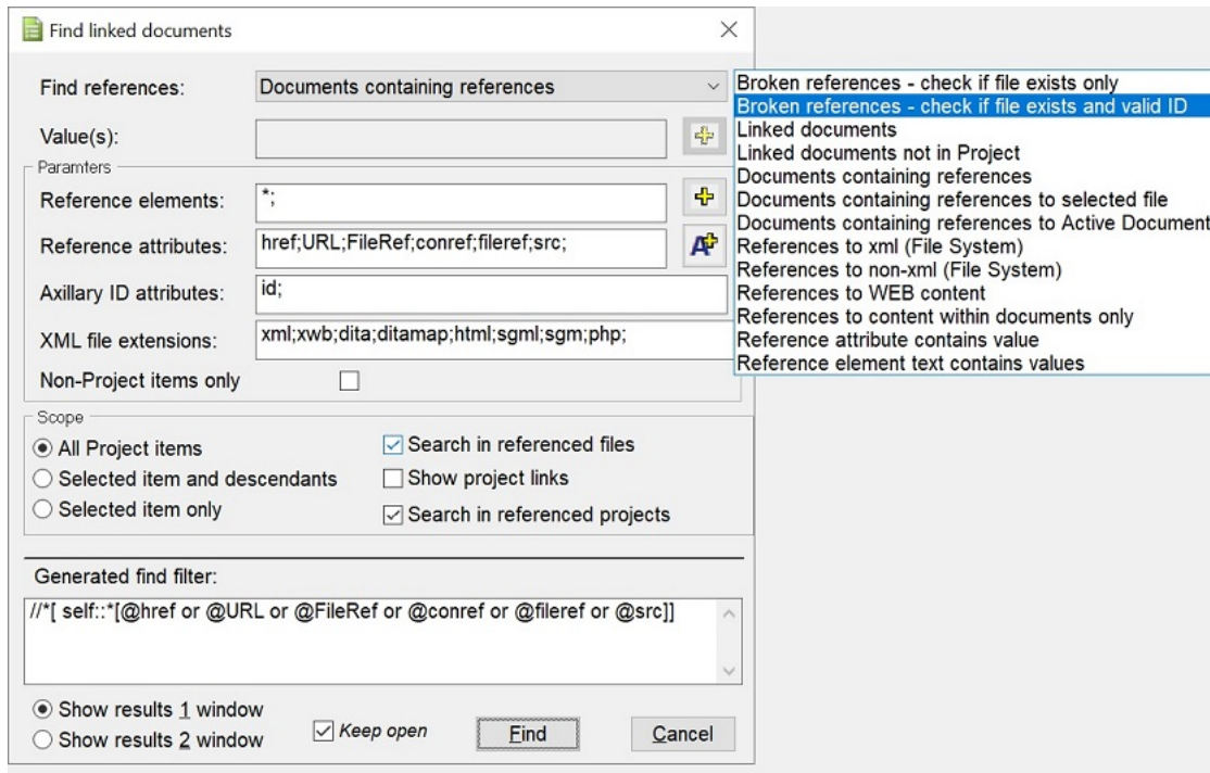
Figure 19: Find and validate links: user interface
