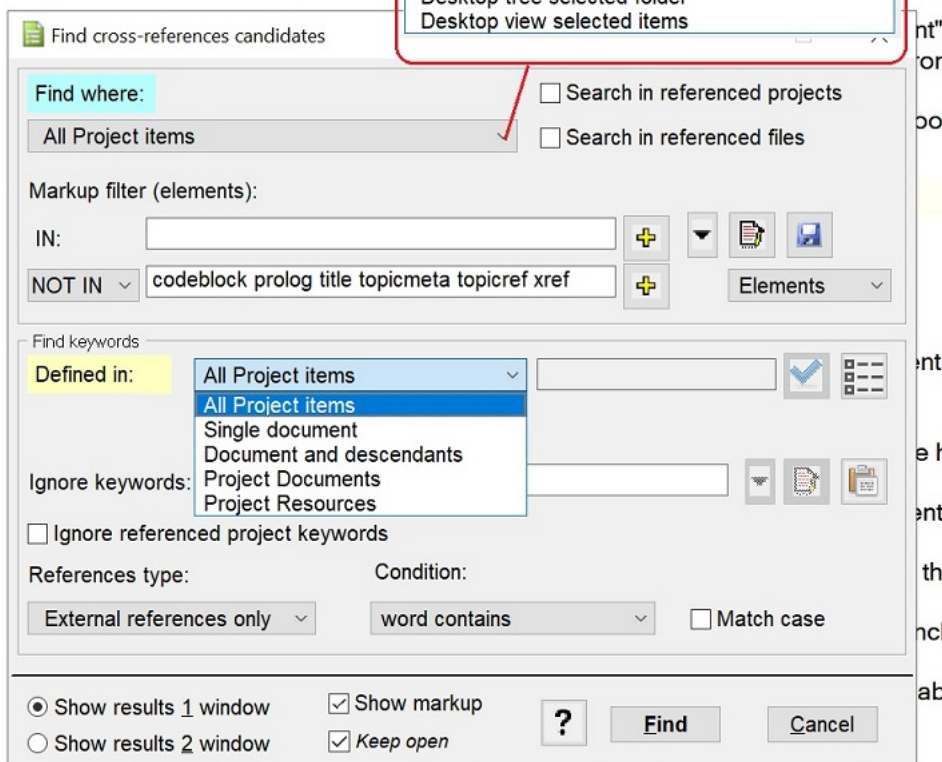
Figure 14: Find cross-references candidates: Find UI
