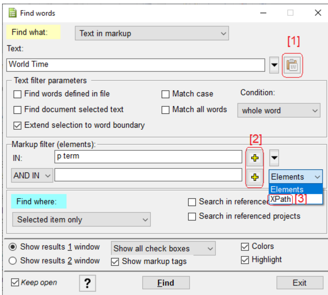
Figure 6: Find Content UI: Advanced markup filtering
