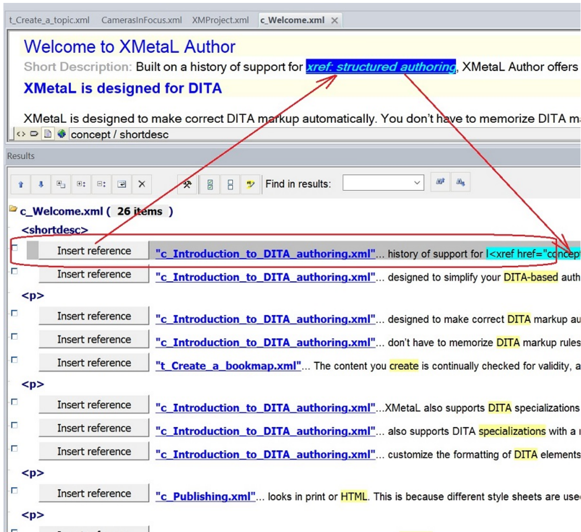
Figure 15: Find cross-references candidates: Set reference UI
