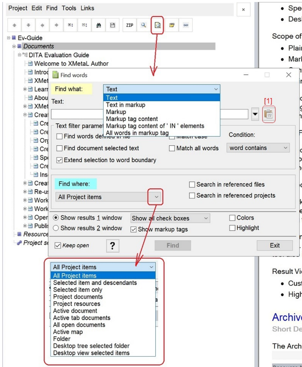
Figure 3: Find Content UI : Main
