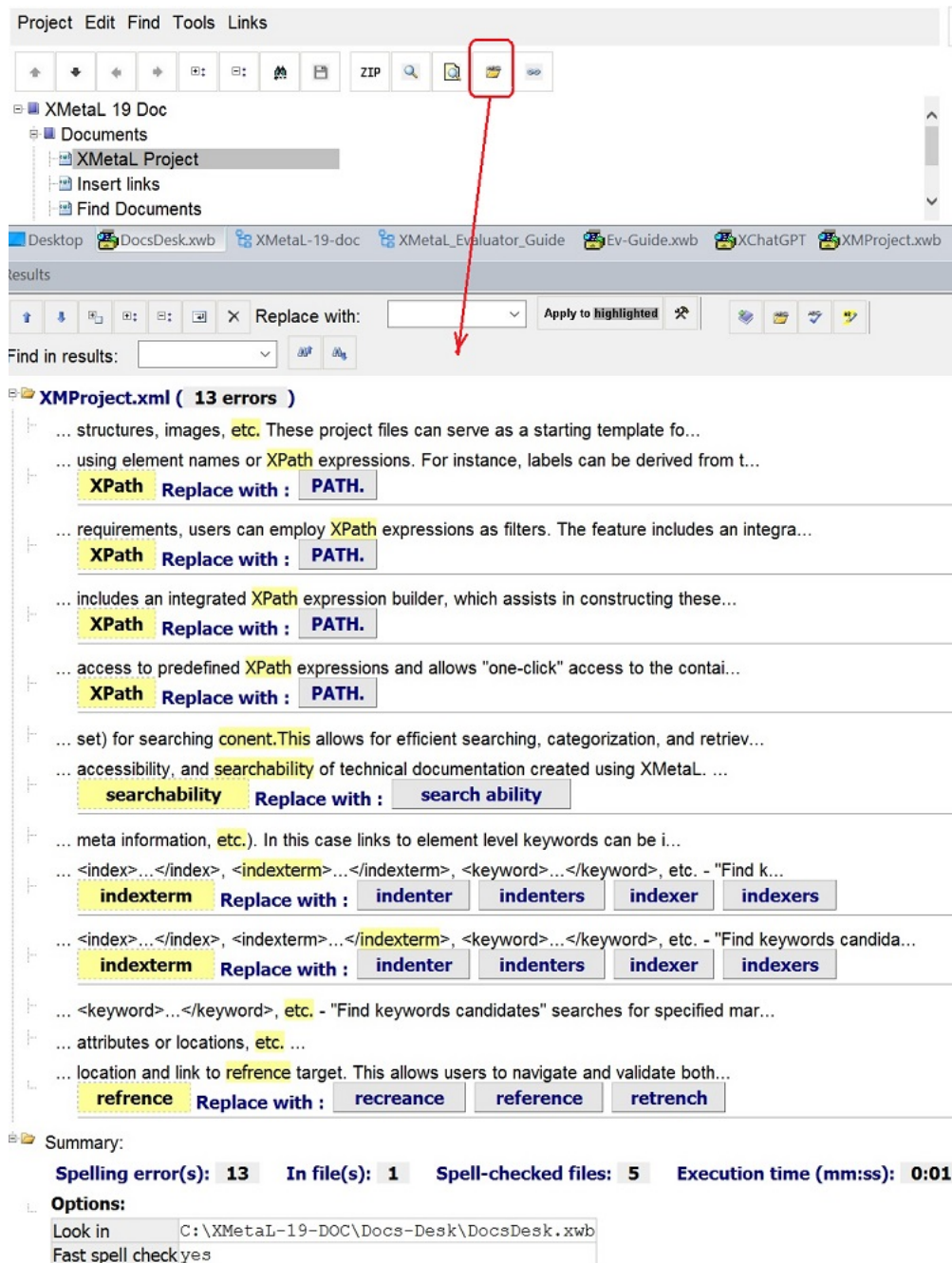
Figure 8: Spell check results tab
