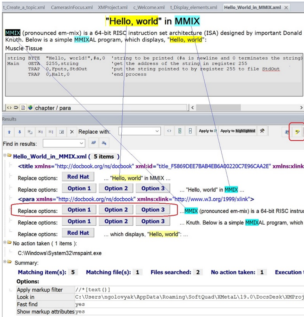
Figure 5: Find Content UI: Keywords in file - Results window with replace options
