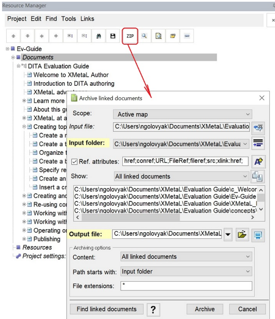
Figure 6: Archive UI
